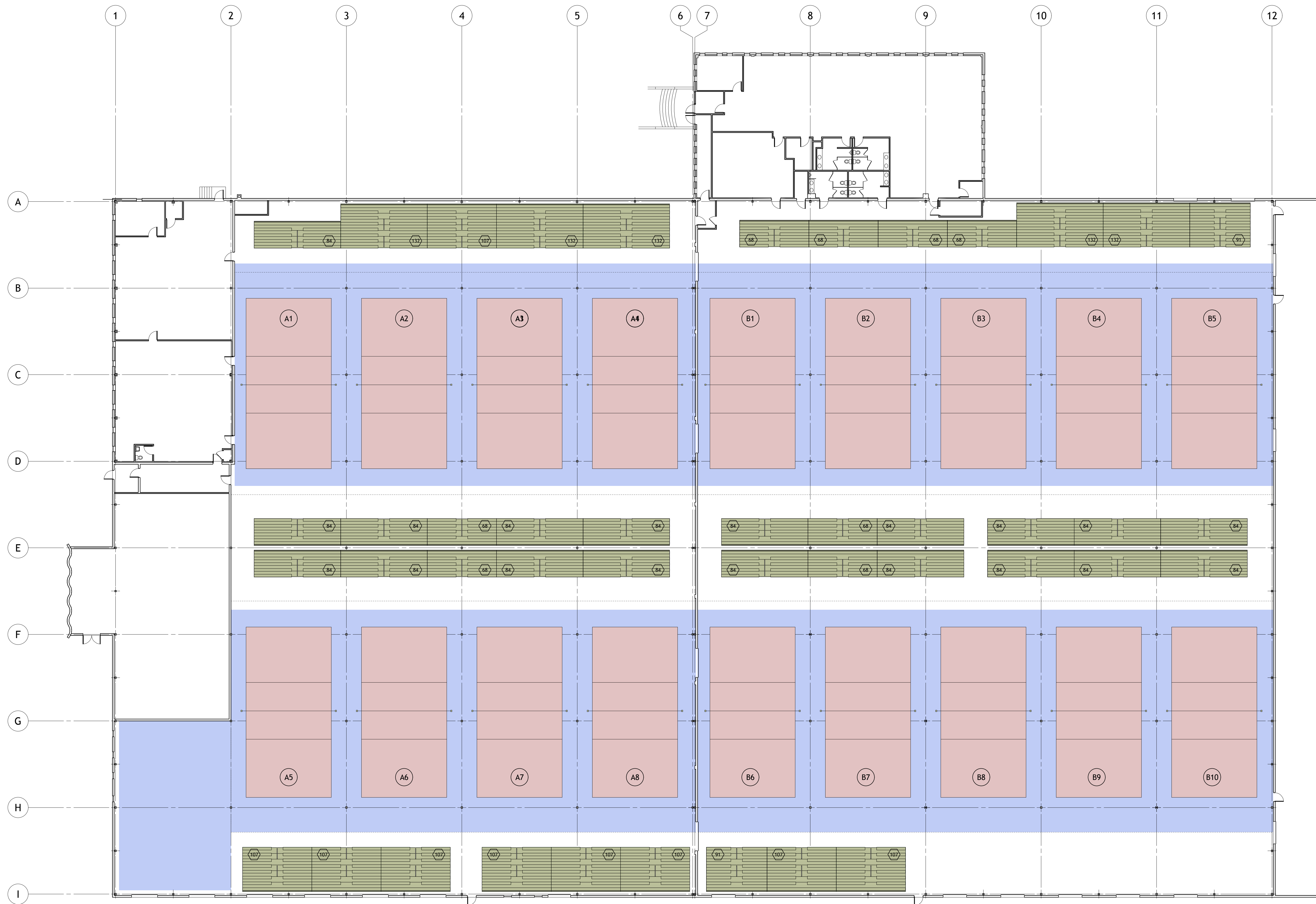
1 FIRST FLOOR PLAN a1 1/16" = 1'-0"
